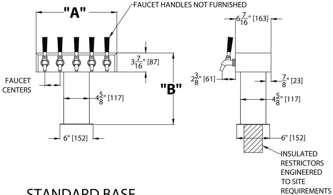
STANDARD BASE TEE TOWERS
